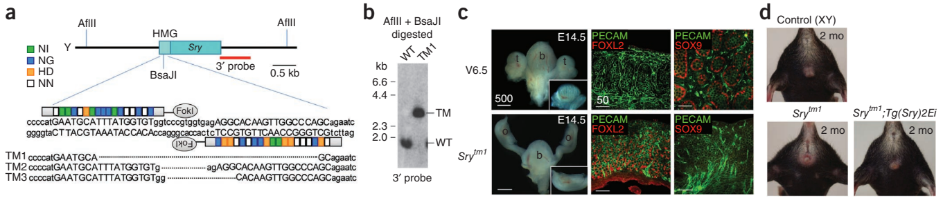
Figure 1 Genetic modification of Sry using TALENs. (a) Schematic of Sry TALEN pair 2 and its recognition sequence in the high mobility group (HMG) domain of Sry . TAL repeats are color-coded to represent each of four repeat variable di-residues (RVDs); each RVD recognizes one corresponding DNA base (NI = A, NG = T, HD = C, NN = G). Nucleotides bound by TALENs are capitalized. Shown below are clones (targeted mutation (TM) alleles 1–3) with Sry deletions indicated by dotted lines. Sry tm4 (540-bp deletion) and Sry tm5 (440-bp deletion) clones are not shown. (b) Southern blot analysis of targeted alleles. AflIII/BsaJI-digested genomic DNA was hybridized with a 3' probe. Expected fragment size: WT = 1.7 kb, TM = 3.2 kb. (c) E14.5 control embryo derived from parental V6.5 mESCs developed as an anatomic male, with testes (t), whereas Sry tm1 embryo developed as an anatomic female, with uterus and ovaries (o). b, bladder. Section of control gonad shows Sertoli cell marker expression (SOX9) and testicular cord formation, whereas section of Sry tm1 gonad shows granulosa cell marker expression (FOXL2). PECAM marks both endothelial and germ cells. Scale bar unit, \mu\text{m} . (d) Sry tm1 -bearing offspring of Sry tm1 females also exhibited female external genitalia and mammary glands (lower left). Anatomic sex reversal of Sry tm1 mice was rescued by the Sry transgene (lower right). (e) Schematic overview of strategy to generate Sry -GFP knock-in alleles. (f) Southern blot analysis of knock-in alleles. AflIII-digested genomic DNA was hybridized with 3' probe or internal GFP probe. Expected fragment size: WT = 3.9 kb, TM(GFP) = 7.0 kb. (g) RT-PCR analysis of GFP transcript expression in tissues from E12.0 Sry -GFP embryos. Internal controls without RT confirmed the absence of genomic DNA contamination. Gapdh was used as reference.
