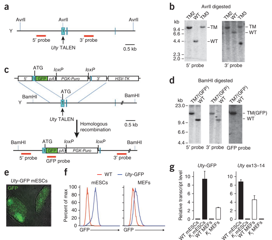
Figure 2 Genetic modification of Uty using TALENs. (a) Schematic overview of targeting strategy. (b) Southern blot analysis of AvrII-digested genomic DNA with 5' probe or 3' probe. Expected fragment size: WT = 4.7 kb (5' probe) and 7.7 kb (3' probe); TM = 12.5 kb for both probes. (c) Schematic overview of strategy to generate Uty -GFP knock-in alleles. (d) Southern blot analysis of BamHI-digested genomic DNA with 5' probe, 3' probe or internal GFP probe. Expected fragment size: WT = 10.4 kb, TM(GFP) = 13.5 kb. (e) Bright field/GFP overlay image shows that Uty -GFP mESCs expressed fluorescent protein. (f) Flow cytometric analysis for GFP fluorescence in Uty -GFP mESCs and MEFs, compared with wild-type counterparts. (g) Quantitative analysis of Uty -GFP and Uty transcript levels in cells by RT-PCR using primers spanning exon 1-GFP (left) and exons 13–14 (right), respectively. K_i = knock-in.
